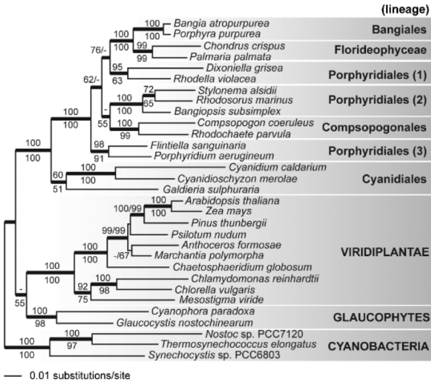
FIG. 1. Bangiophycean red algal phylogeny inferred using the maximum likelihood (ML) method and the combined plastid protein sequences of PSI P700 chlorophyll a apoprotein A1, PSI P700 chlorophyll a apoprotein A2, PSII reaction center protein D1, PSII 44 kD apoprotein, PSII D2 reaction center protein, RbcL, and TufA. The results of a ML bootstrap analysis are shown above the branches, whereas the values below the branches result from a maximum parsimony bootstrap analysis. The thick branches represent >95% Bayesian posterior probability.
